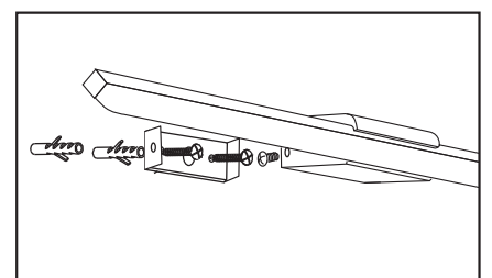
A pared / Wall fixing
